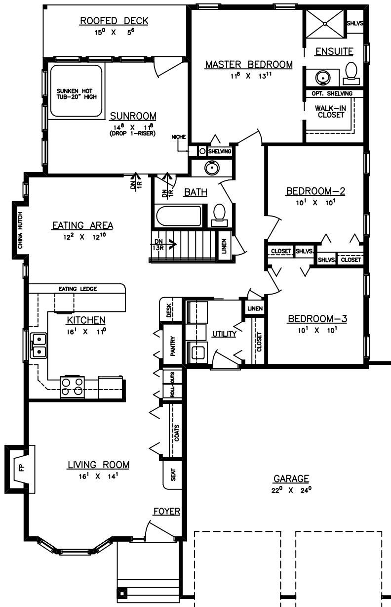
FLOOR PLAN
